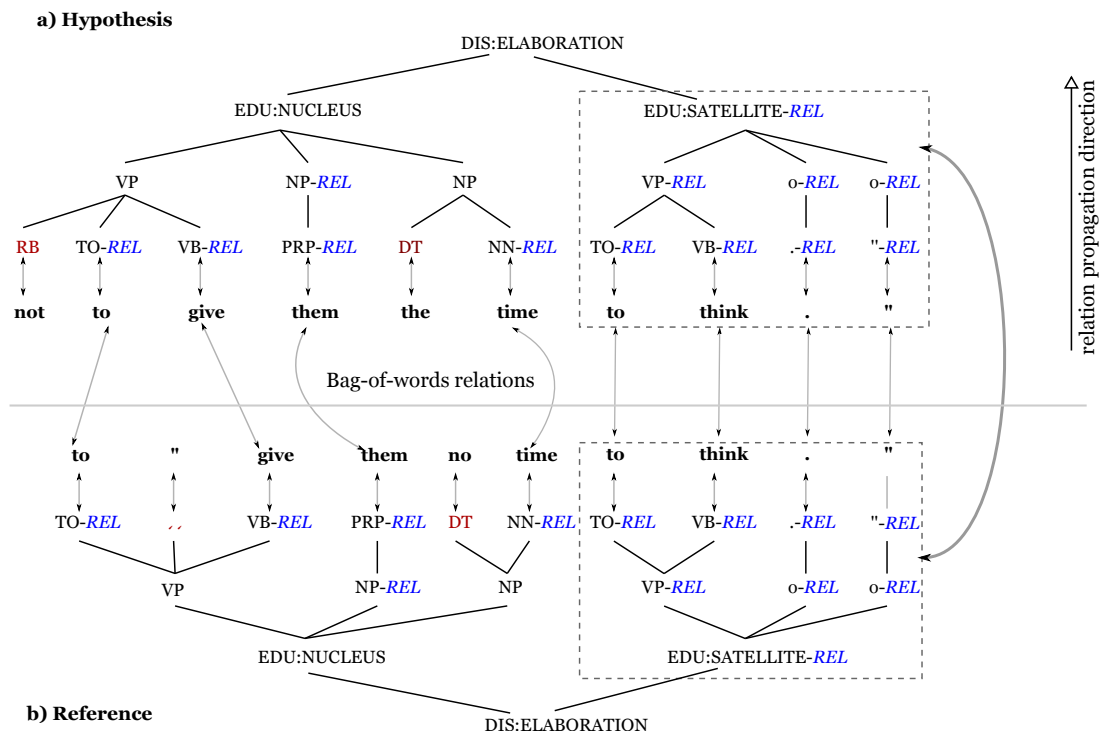
Figure 1: Hypothesis and reference trees combining discourse, shallow syntax and POS.
