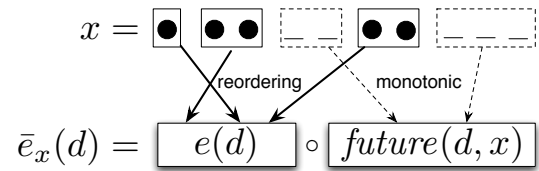
Figure 3: Example of the extension function \bar{e}_x(\cdot) (and future string) on an incomplete derivation d .
