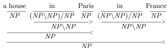
(a) A standard derivation of a house in Paris in France , with a dependency from in France to house
